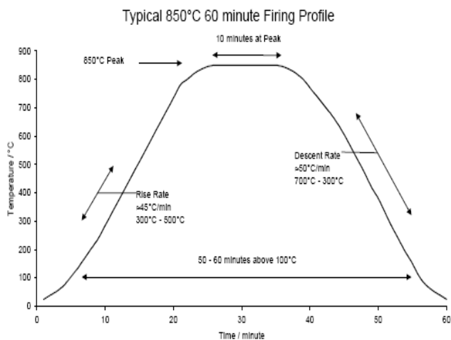
CHART 1. FIRING PROFILE
